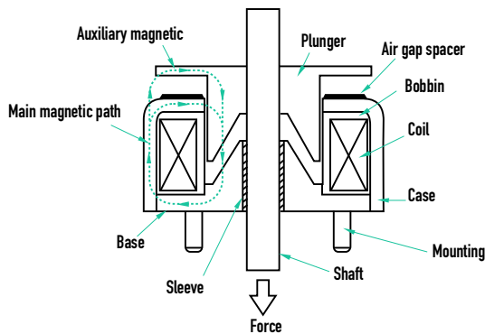
Fig. 1 Conical pole
